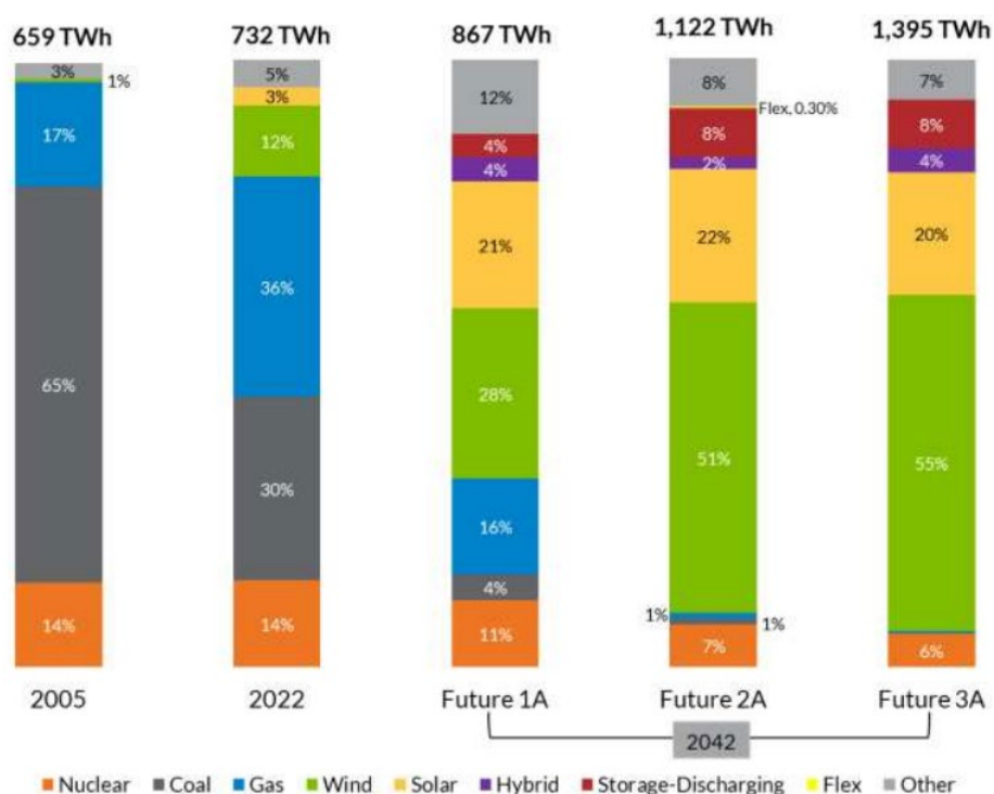
Figure 4 – Overview of MISO's Generation Fleet Mix Transition in Futures Series 1A
